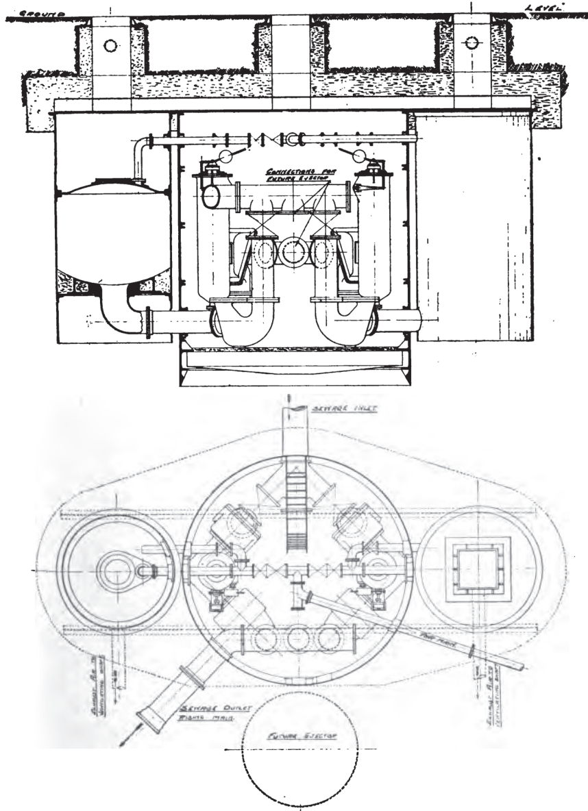
Fig. 37c. "Coombs" Pneumatic Ejector.
