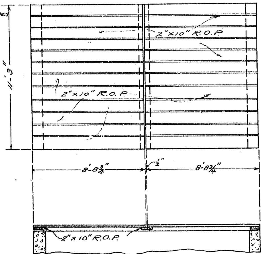
PLAN AND SECTION OF COVER FOR IMHOFF TANK. SCALE 1"=4'
