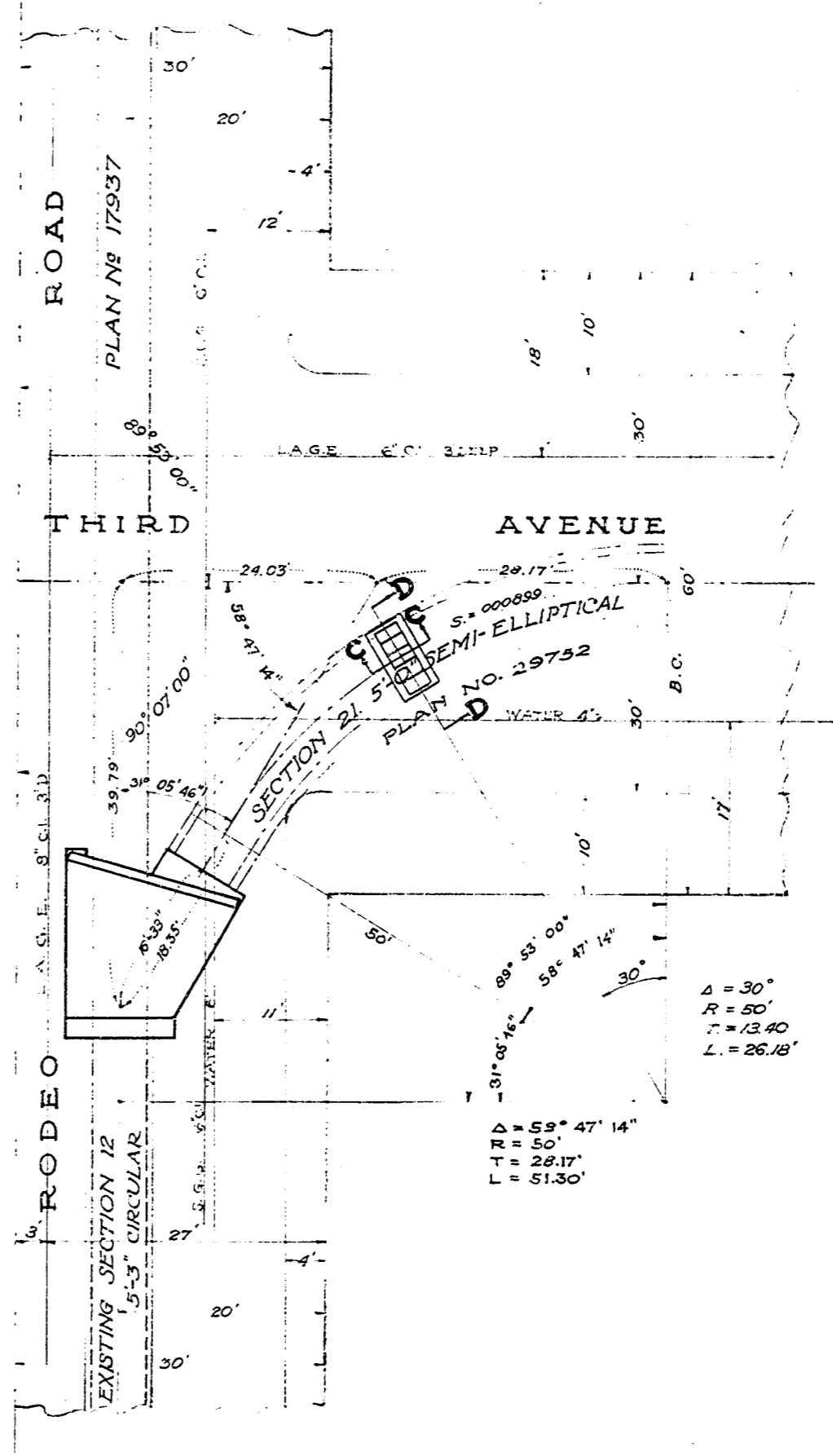
LOCATION PLAN Scale: 1"=10'
