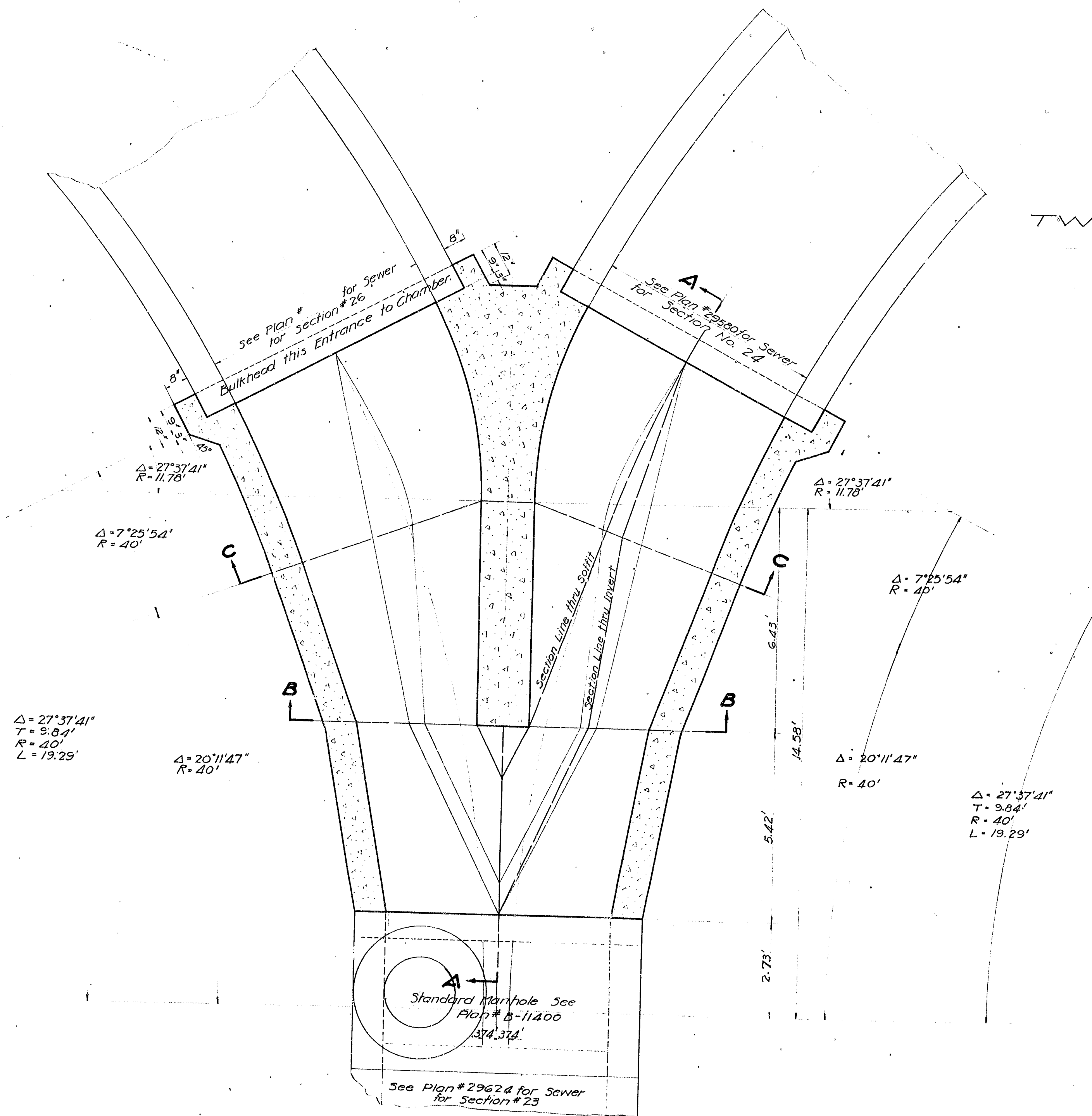
SECTIONAL PLAN Scale 1/2"=1'-0"
