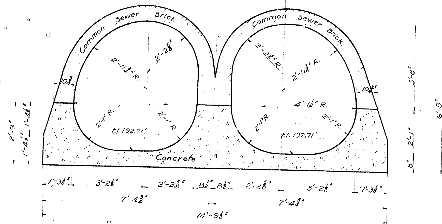
SECTION C-C Scale 1/2"=1'-0"
