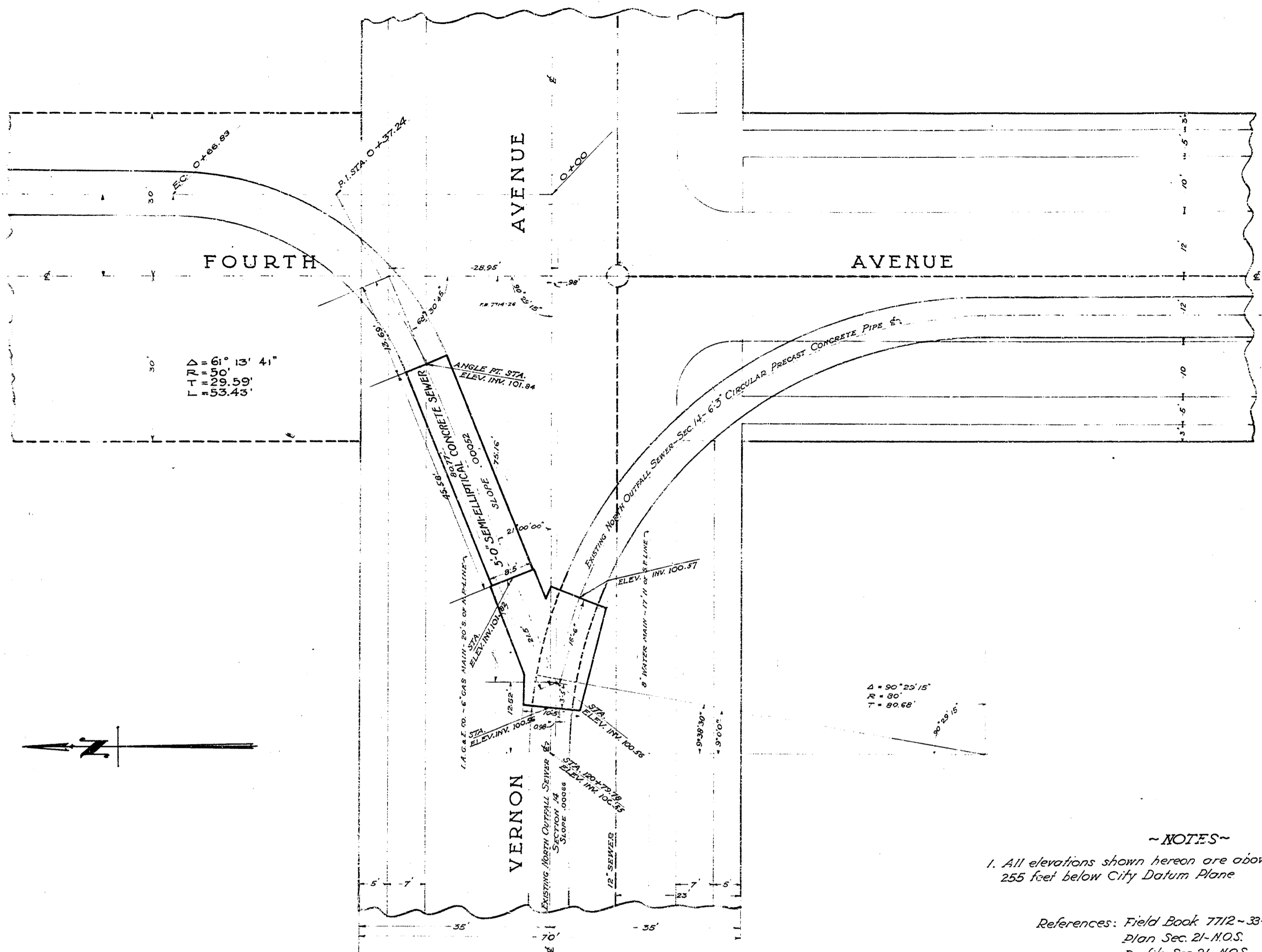
LOCATION PLAN Scale: 1" = 10'
